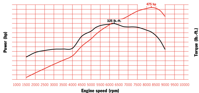
911 GT3: 475 hp at 8,250 rpm, 325 lb.-ft. at 6,250 rpm
